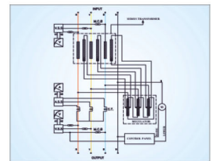
Basic Circuit
