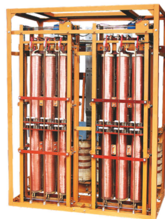
Inner View of a 2000 KVA Stabilizer
