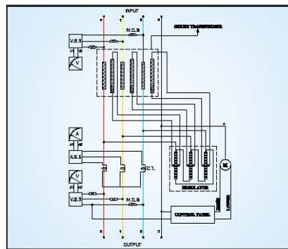
Basic Circuit
